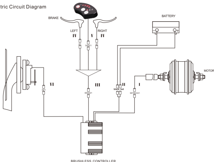
Electric Circuit Diagram
